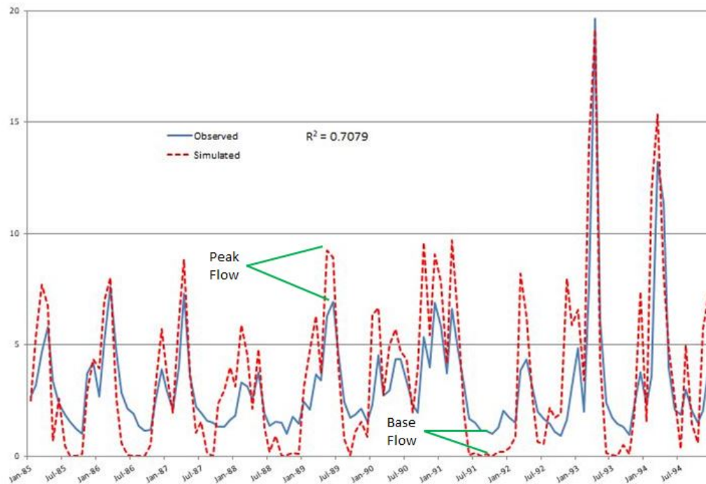
Figure 3. Pre-Calibration Observed and Simulated Houserville Stream Gage Flow Data (stream flows are in units of water depth [cm] over the watershed)
